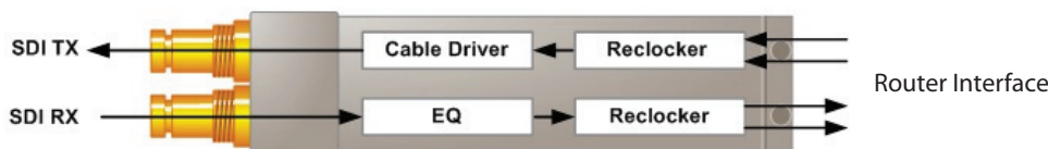
Functional Coaxial SFP Diagram
